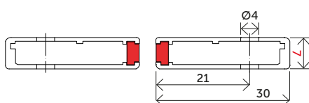
Mechanical profile
