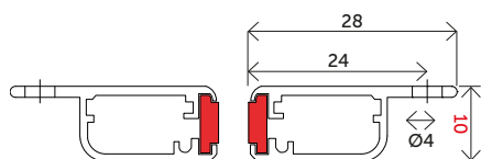
Mechanical profile
